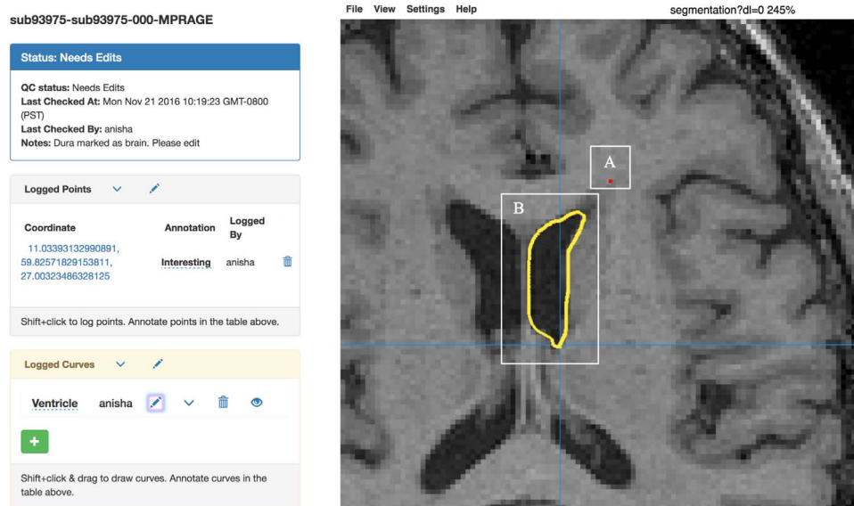
Fig. 6. The annotations panel can be used to annotate a single point (shown in red, part A) and curves (shown in B). When annotating points, the user is shown the selected x,y,z world coordinates and is able to name the annotation. In the curve annotation panel on the left sidebar, the user is able to name the curve and add/remove curves. Keyboard shortcuts: “dd” removes the previous annotation and “zz” toggles the segmentation overlay.
